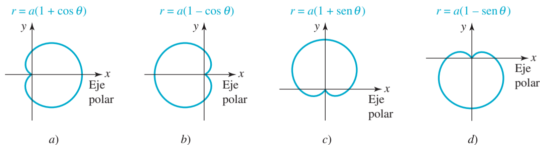
FIGURA 12.2.6 Cardioides
